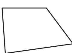
Quadrilateral (4 sides)
