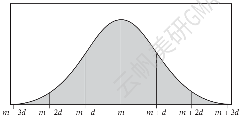
Normal Distribution
