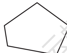
Pentagon (5 sides)
